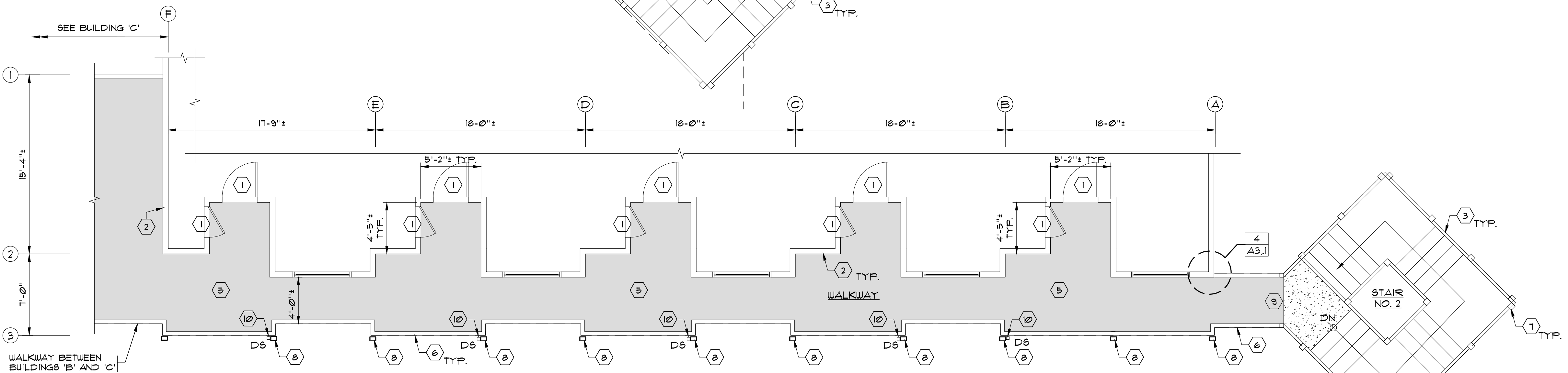
WALKWAY PLAN AT BUILDING 'B' SCALE: 3/16" = 1'-0"
