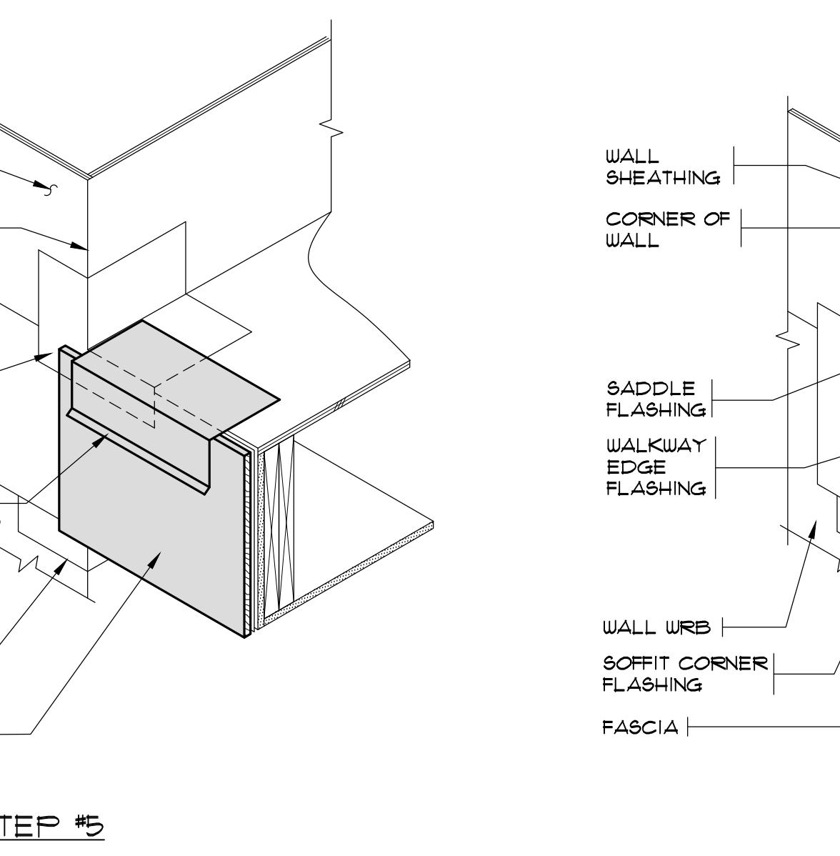
TYPICAL WALKWAY SADDLE FLASHING AT WALL CORNER 4 SCALE: N.T.S.
