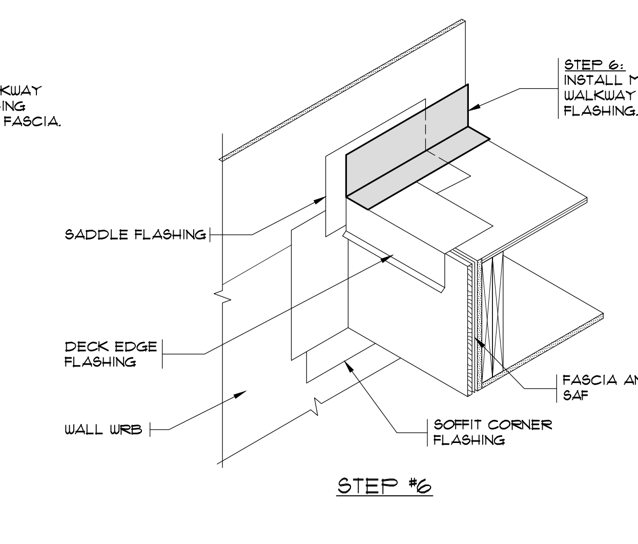
TYPICAL WALKWAY SADDLE FLASHING AT FLAT WALL 1 SCALE: N.T.S.
