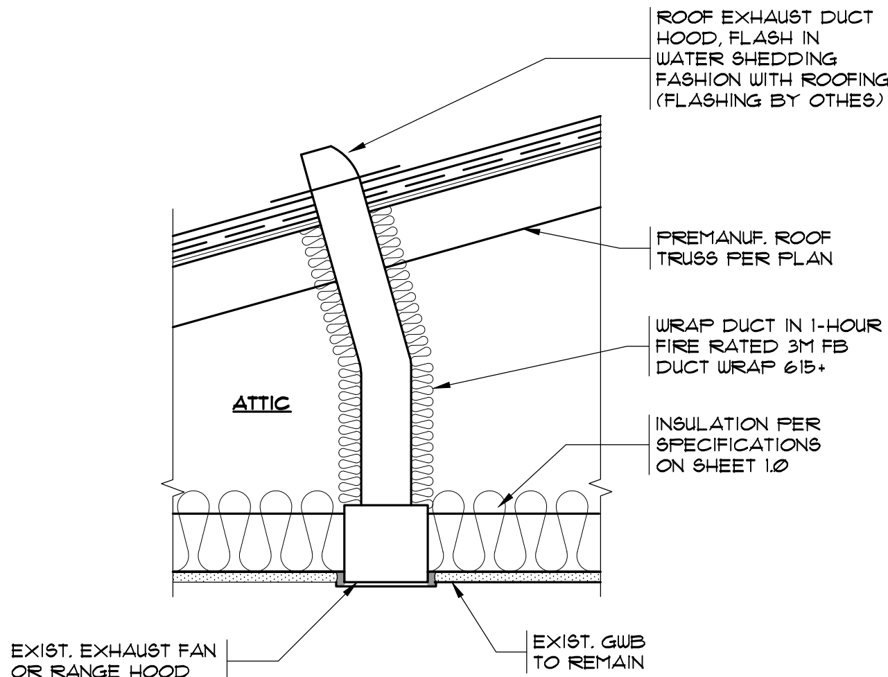
TYPICAL EXHAUSE FAN ASSEMBLY SCALE: 1 1/2" = 1'-0"
