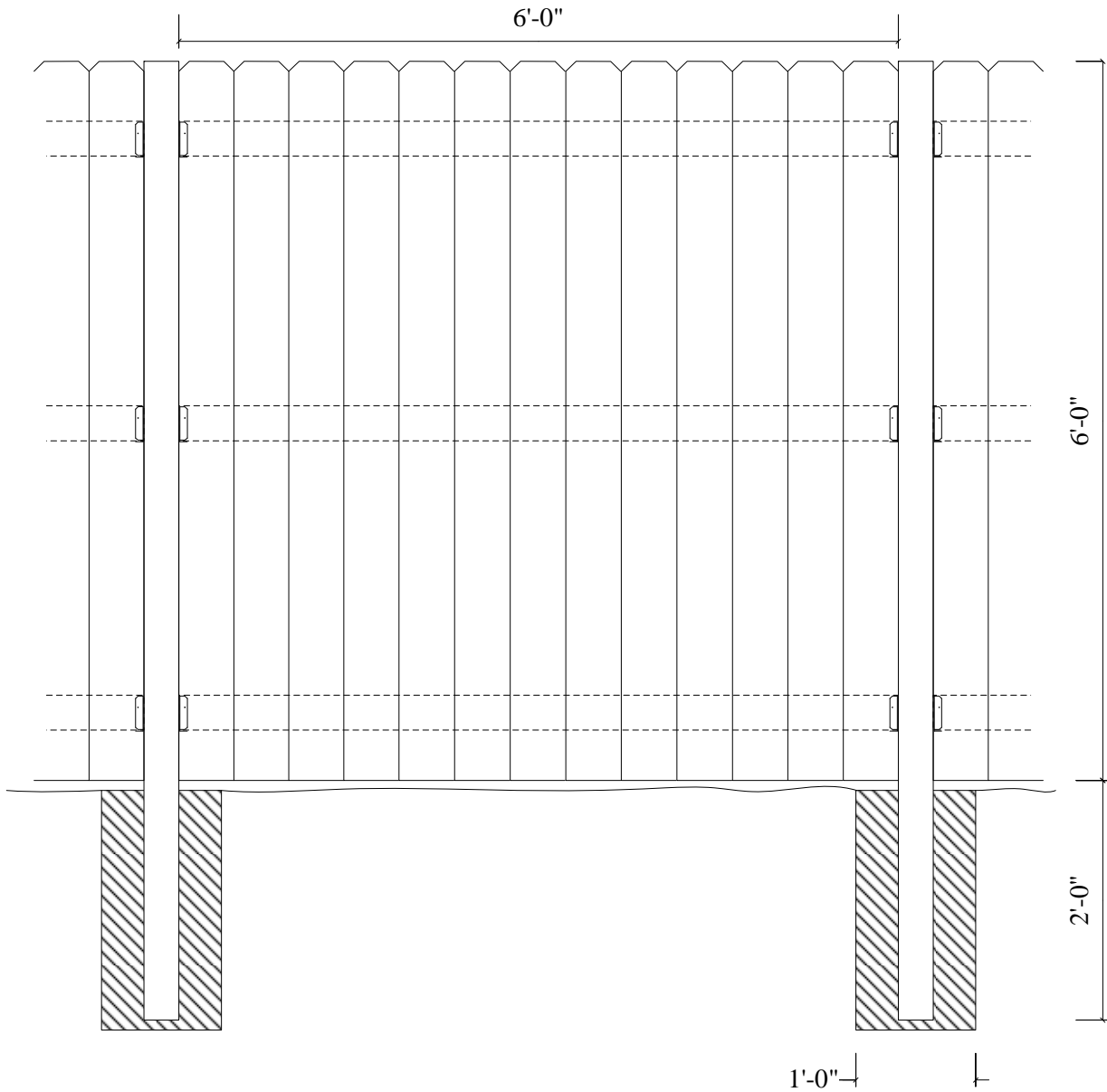
TYPICAL FENCE PANEL
